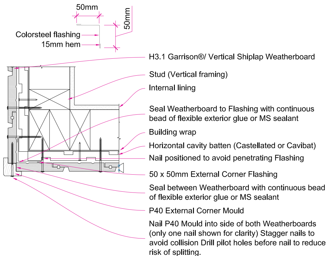
Figure 1.17 Cavity fixed – external corner
